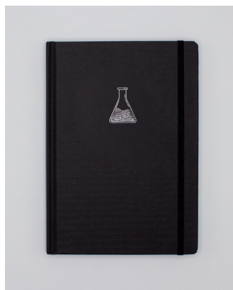
Chemistry
