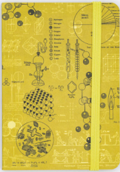
Chemistry: Models
