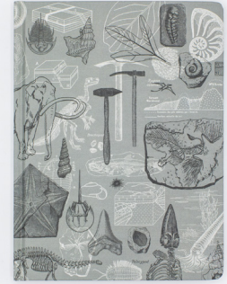
Paleontology - Lined
