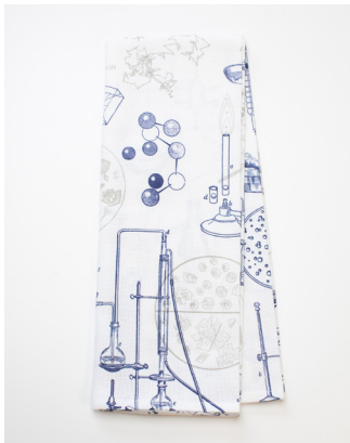
Chemistry
