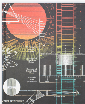
Sol: Spectra
