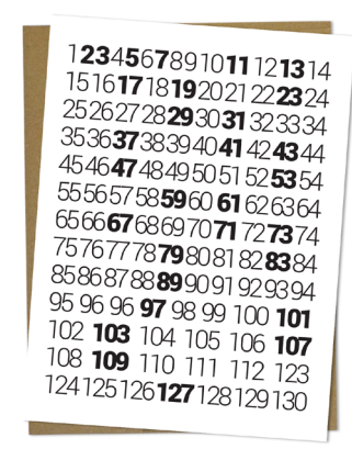
Prime Numbers
