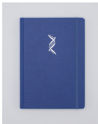
DNA
