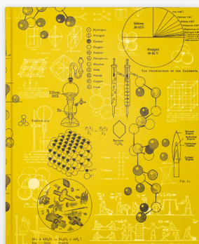
Chemistry Models
