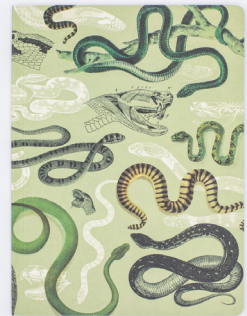
Snakes - Dot
