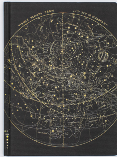
Astronomy
