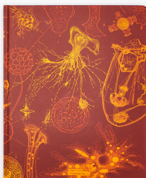
Microbiology
