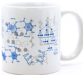
Genetics DNA
