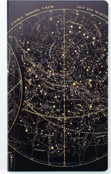
Astronomy
