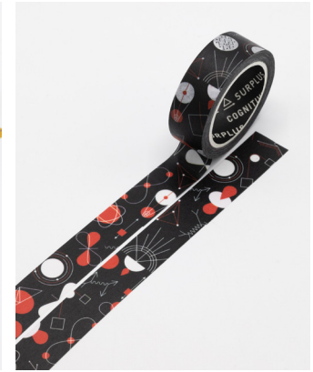
Physics
