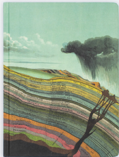
Earth's Geology
