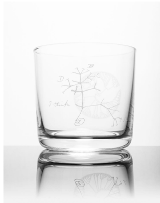
Phylogenetic Tree
