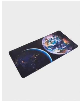
Day & Night on Earth
