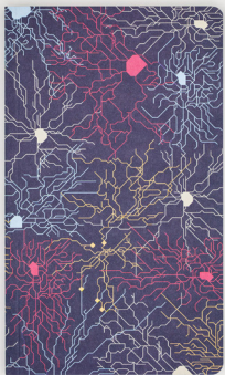
Neural Circuit
