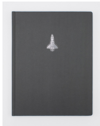
Astronautical
