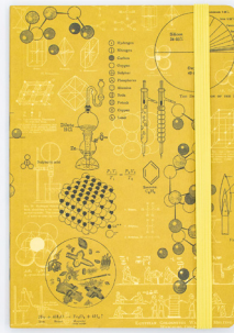
Chemistry: Models
