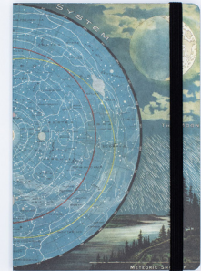
Star Map
