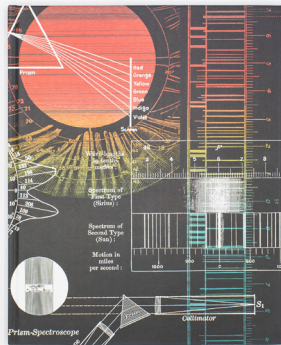
Sol: Spectra
