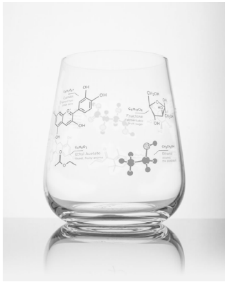
Wine Chemistry
