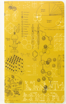
Chemistry Models
