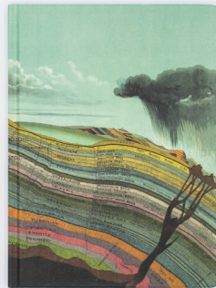
Earth's Geology
