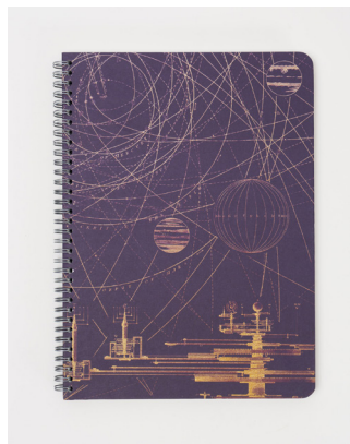
In Orbit
