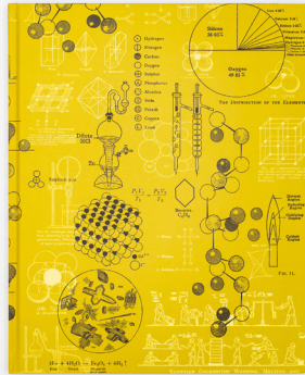
Chemistry Models
