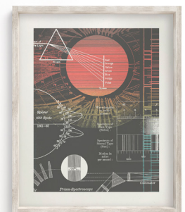
Sol: Sun
