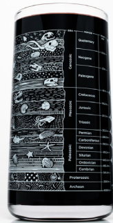
Core Sample
