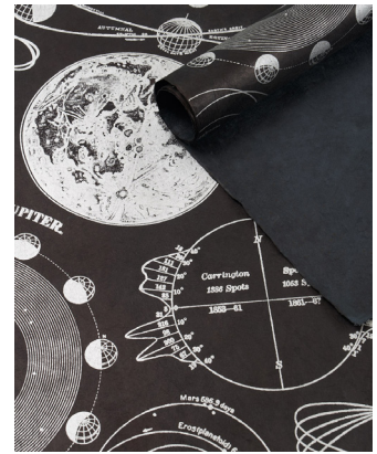
Solar System
